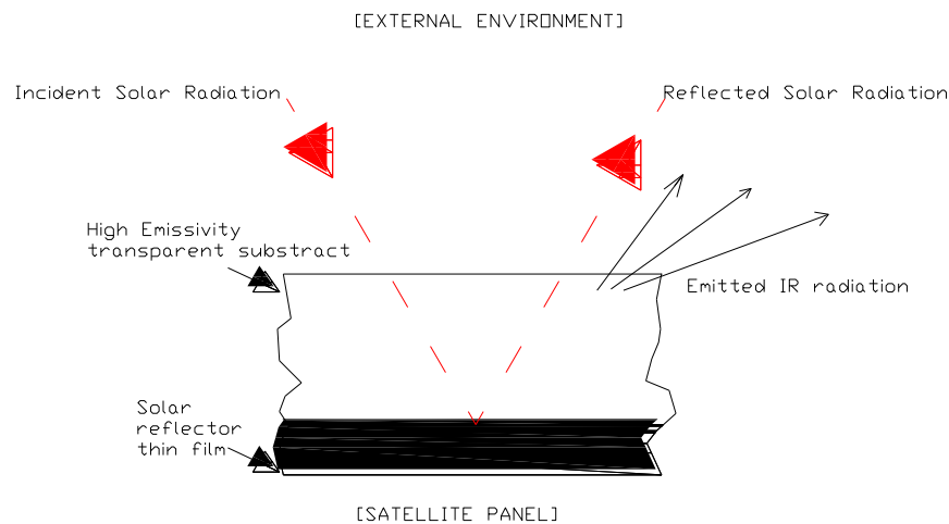
Figure 4. Second Surface Mirror (SSM).
