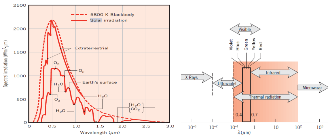
Figure 3. Solar radiation spectra in Earth's orbit. Adapted from Bergman and Lavine (2017).
