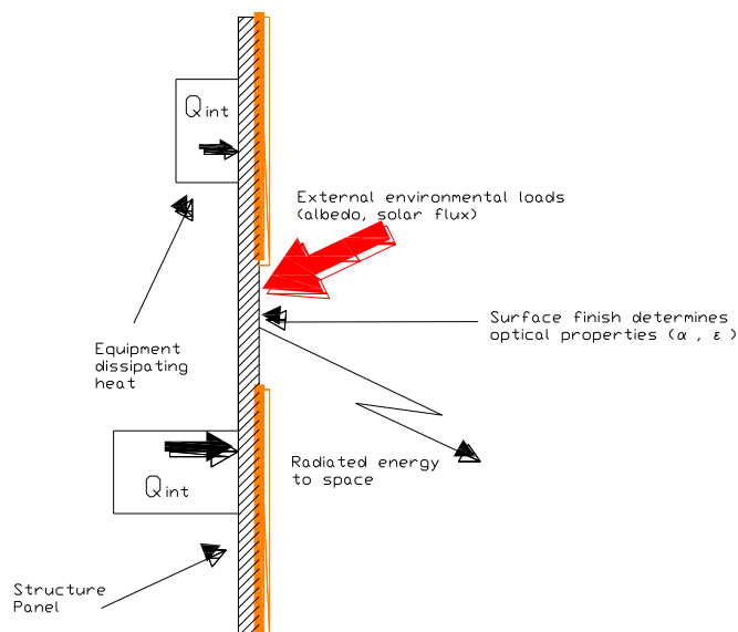
Figure 2. Simple radiator mounted in a satellite panel.
