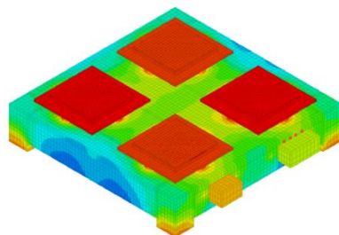
Figure 7. Experiment's TMM with temperature map relative to an arbitrary condition.
