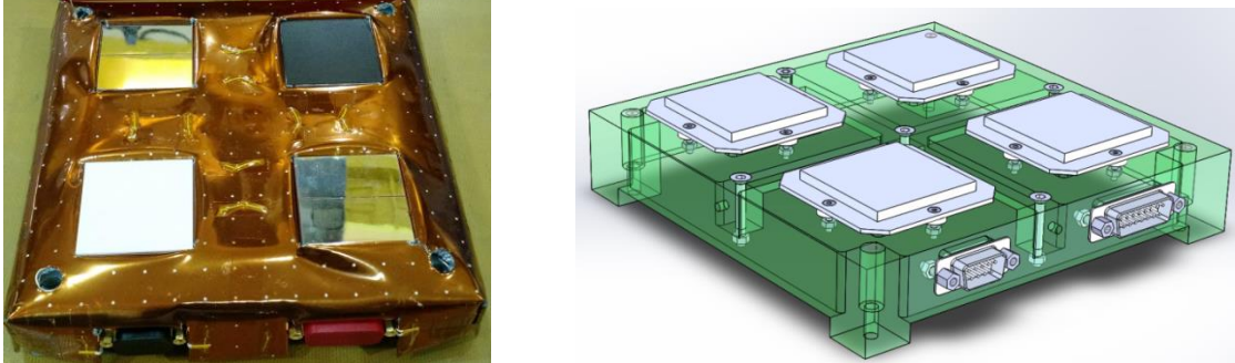
Figure 5. OSR degradation experiment assembly and its mechanical model.
