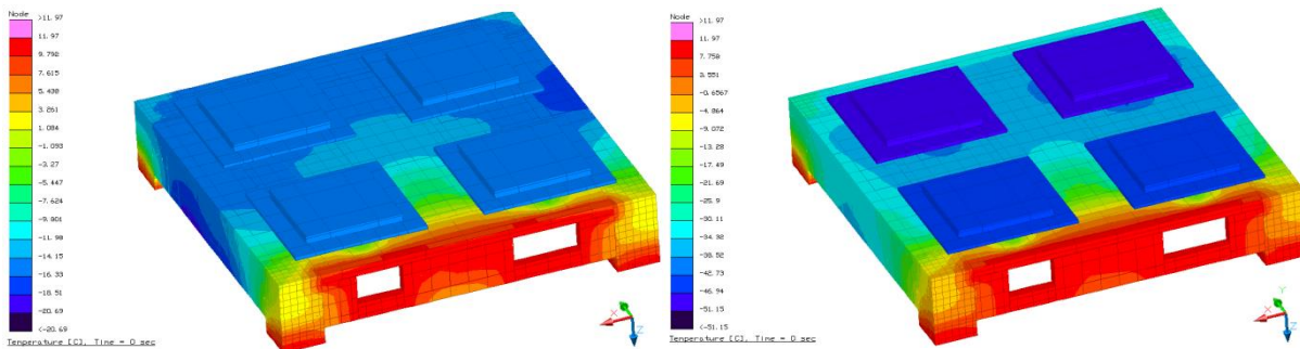
Figure 8. TMM temperature maps for heaters on and off conditions, respectively.
